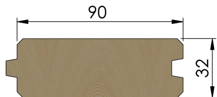
Lames 90x32 mm (1)
