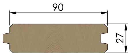
Lames 90x27 mm (1)
