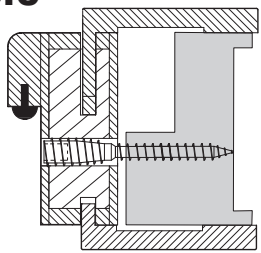
Aspect gâche sur montant strike appearance on frame
